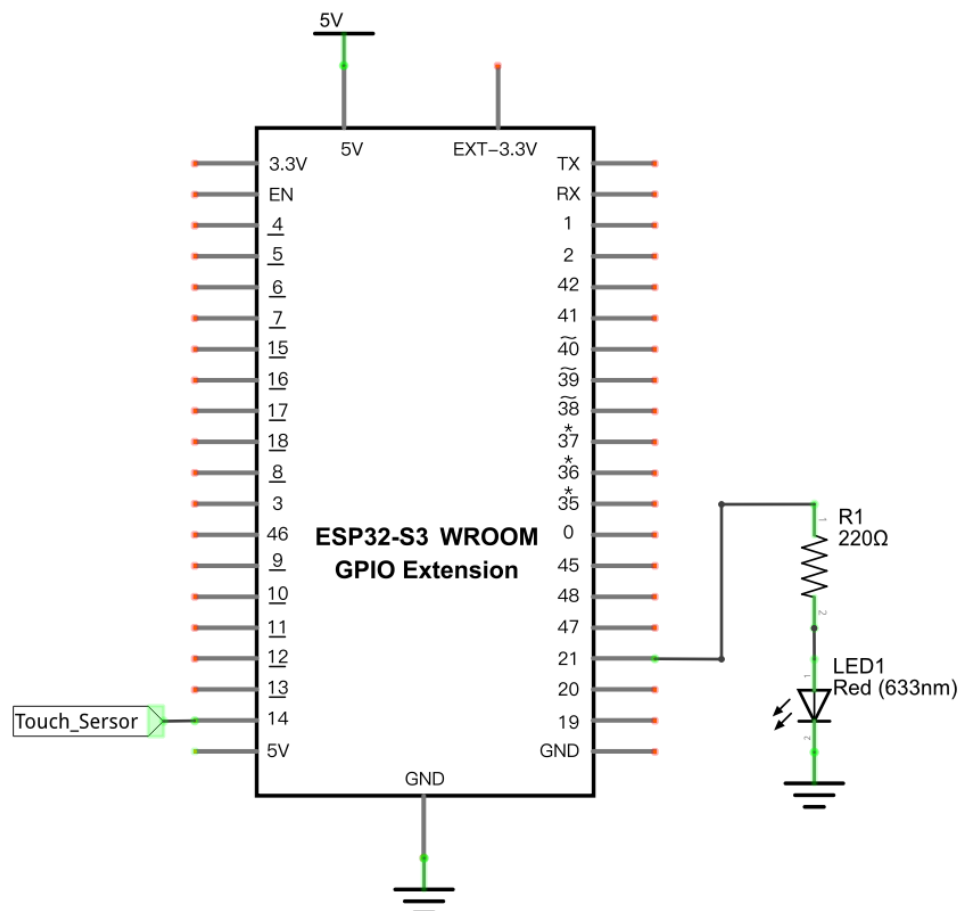
Schematic diagram
