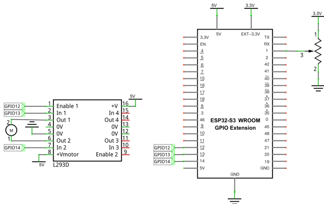
Schematic diagram
