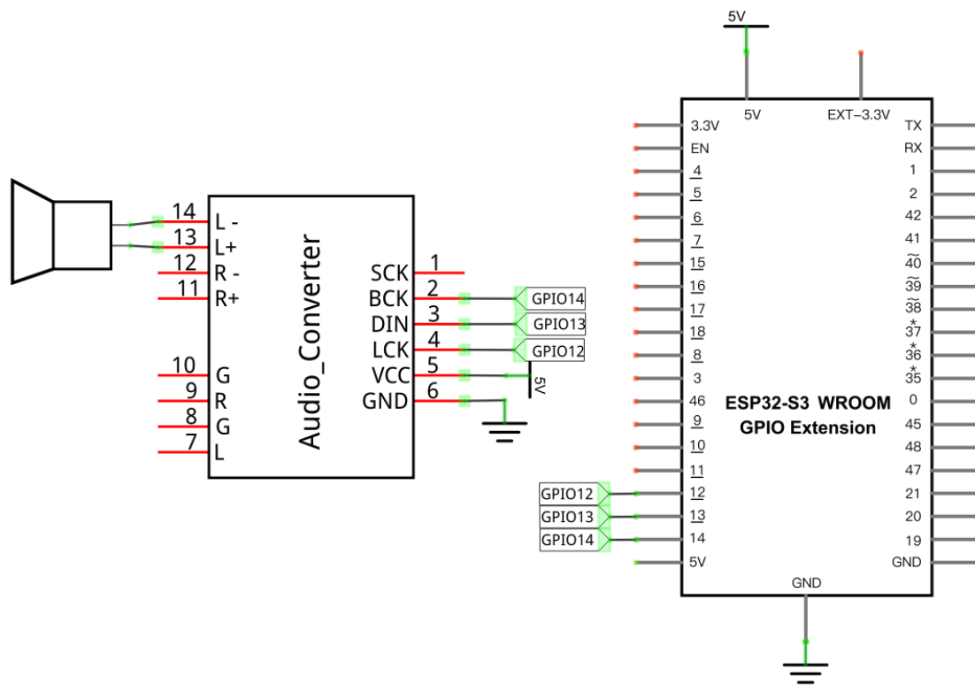
Schematic diagram
