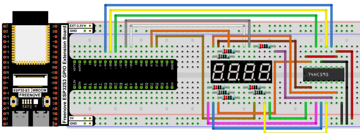
Hardware connection:
